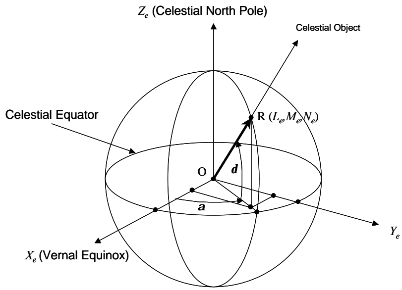
Figure 4-2 Equatorial Coordinates
