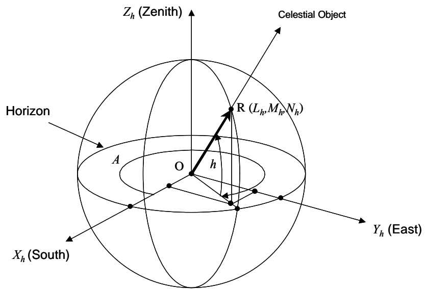
Figure 4-3 Altazimuth Coordinates
