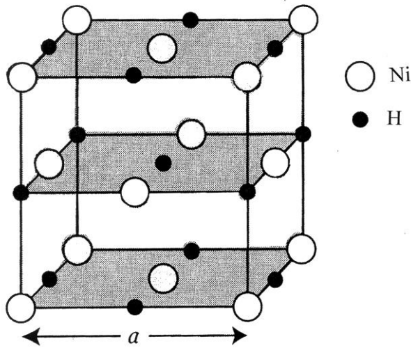
Fig. 2 Atomic arrangement in nickel hydride crystal. Ni(O) atoms locate at corners and centers of faces of a cube with an edge of length a . Hydrogens (●) locate at octahedral interstices (interstitial sites) surrounded by six Ni atoms in this case. (Another interstices surrounded by four Ni atoms are called tetrahedral sites.) The lattice constant a is 3.731 \text{ \AA} = 373.1 \text{ pm} .
