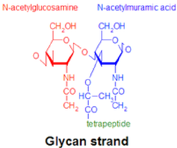
Fig. 14 Molecular structure of glycan strand (after Wikipedia)
