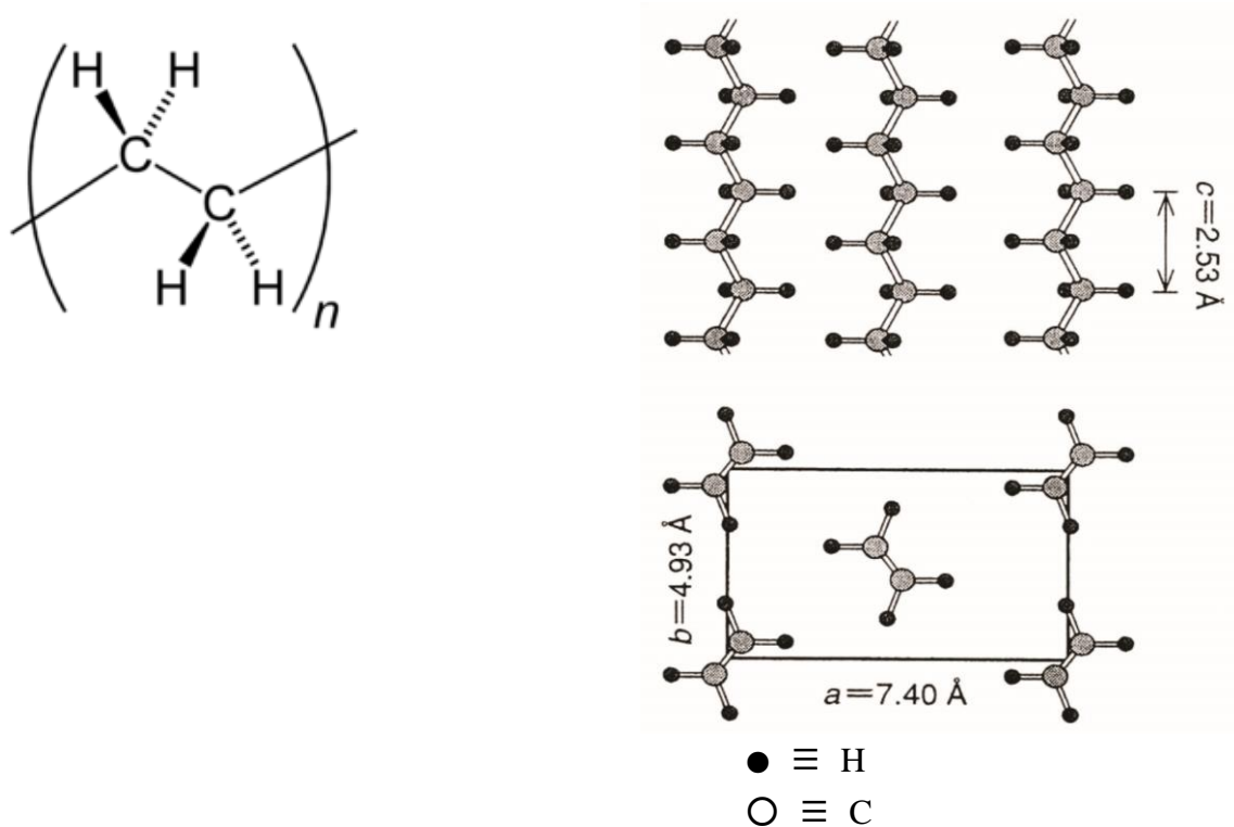
Fig. 5 Lattice structure of XLPE orthorhombic lattice with lattice constants, a = 7.40 \text{ \AA} (740 pm), b = 4.93 \text{ \AA} (493 pm), c = 2.53 \text{ \AA} (253 pm) [Kozima 2010 (Fig. 5)].
